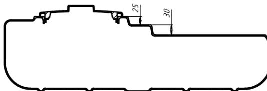
CROSS-SECTION A-A SCALE 1:4
